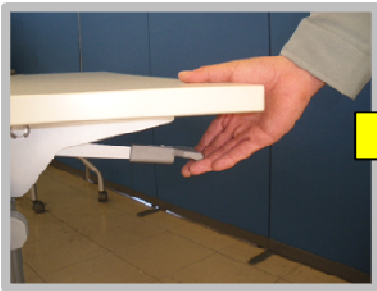
Easy and smooth one-handed operation of flip mechanism. The lever is equipped under the top on both sides.
